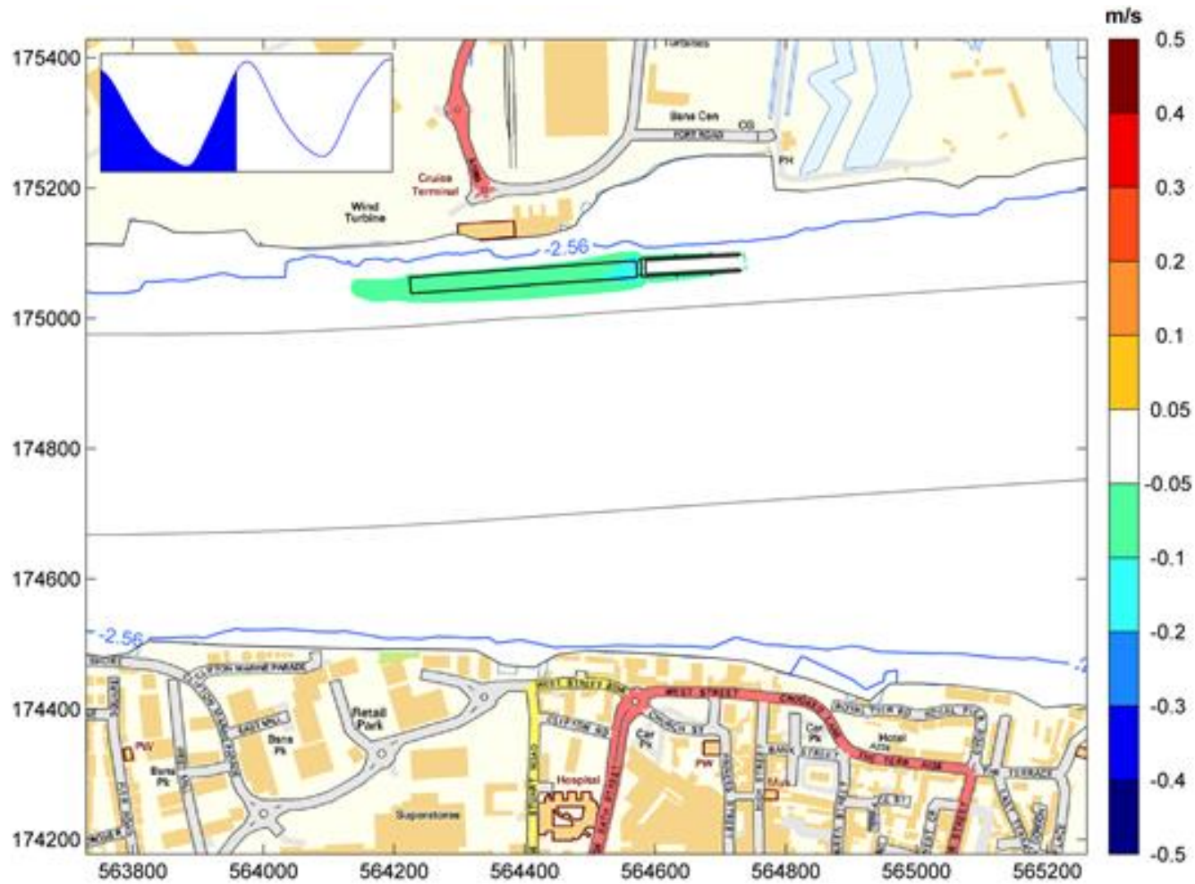
Figure 17.30: Essex Project Site difference in current magnitude at time of peak flood tide against the baseline model.
